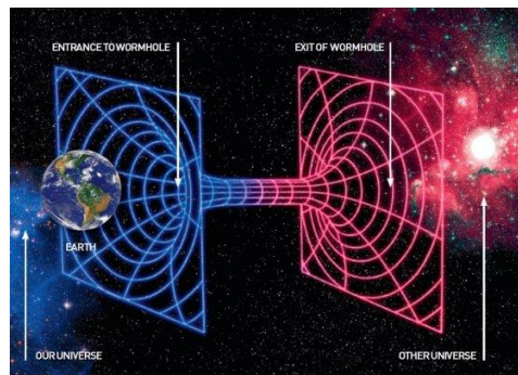
Figure 7 Are wormholes the solution?
