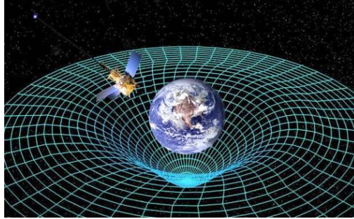
Figure 10 Satellite orbiting Earth is guided by the spacetime curvature generated by the Earth's mass (Photo: NASA)
